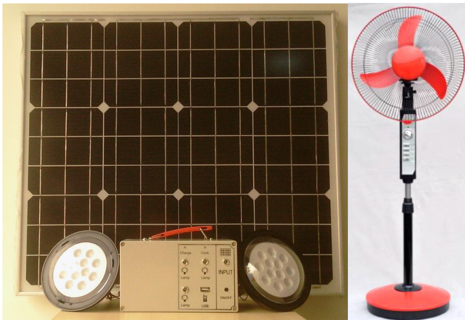
RS-SYS12-9 with 2 X 3 W LED lights bulbs and one 15W solar fan Model RDC16 and mobile with 50 W solar panel
